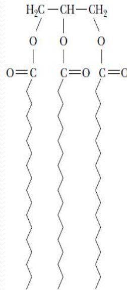
Tristearin (a simple triacylglycerol)
